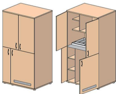
30Н011 840X640X1831
