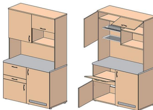
30Н014 1186X600X2173
